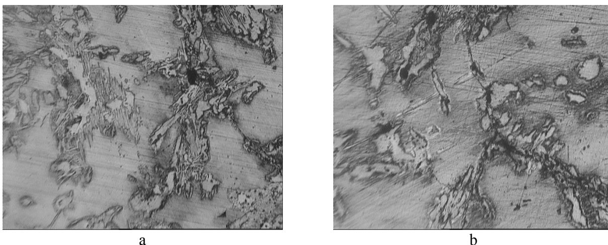
Fig. 2. Microstructure of alloy 110H13L x 100 : a – initial alloy; b – alloy processed by electric current
