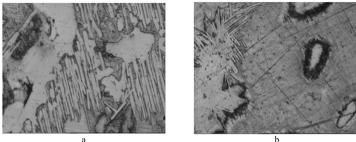
Fig. 3. Microstructure of alloy 110H13L x 500 : a – initial alloy; b – alloy processed by electric current
